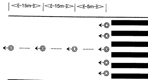
Figure 1 Placement of warning lights – not to scale
